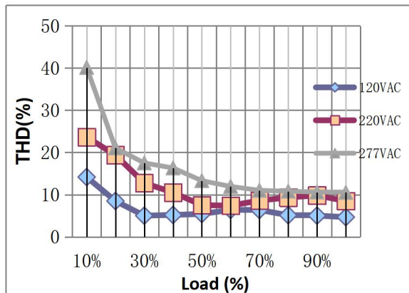
Total Harmonics Vs Different Loads
