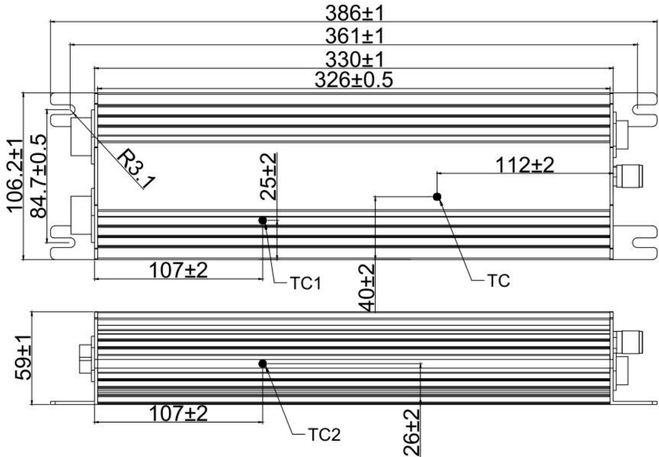
-CJJ3/-CLL3/-CQQ3/-CJJW/-CLLW/-CQQW Model Mechanical Drawing
