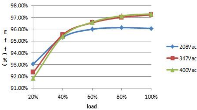
Eff VS load(363Vdc 1.1A)
