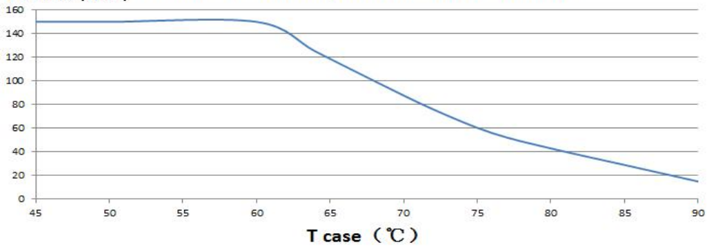
Life time (K hrs) Lifetime VS case temperature@400Vac full load
