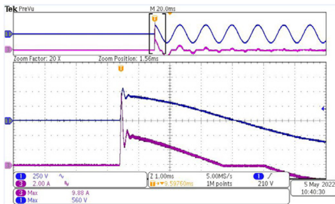
Inrush current
