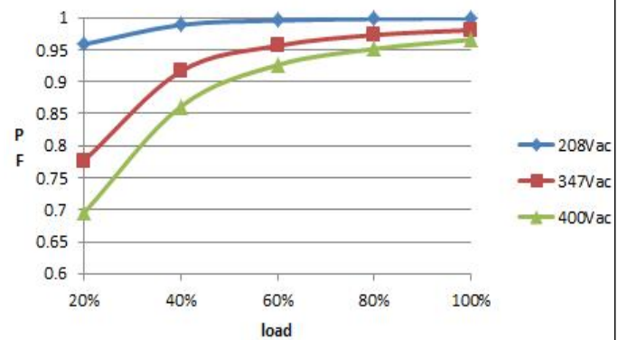
PF VS load(363Vdc 1.1A)
