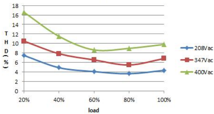
THD VS load(363Vdc 1.1A)
