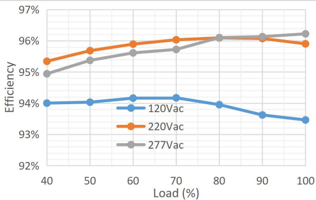
Efficiency Vs Different Loads (Vo=230V Io=1.05A)
