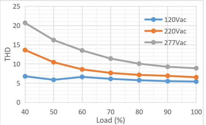
THD Vs Different Loads (Vo=230V Io=1.05A)
