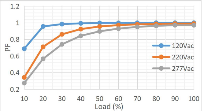
Power Factor Vs Different Loads (Vo=230V Io=1.05A)
