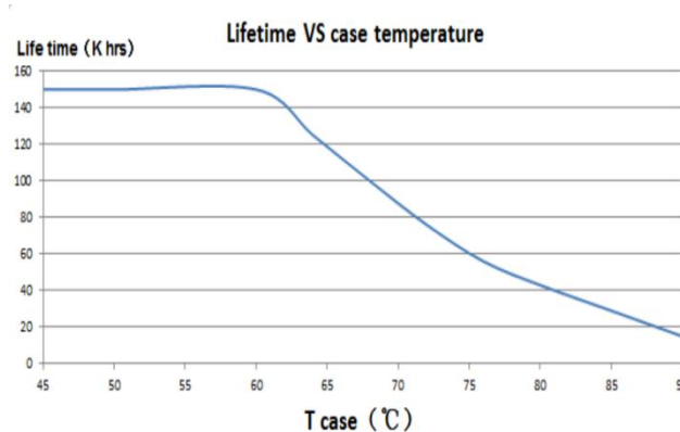
Life Vs Case Temperature
