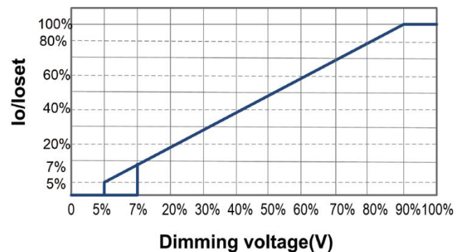
I_o/I_{o\text{set}} vs. Dimming voltage
